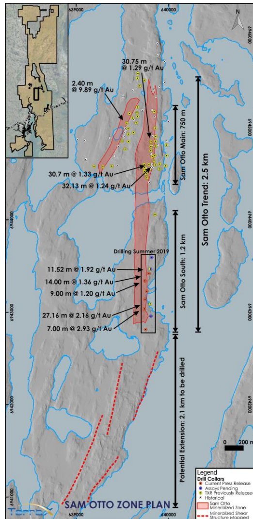
Figure 1: Sam Otto "Mineralized Zone" is defined by drilling and gold bearing surface sampling. Dotted line indicating "Mineralized Shear Structure Mapped" shows the location of favorable extensions of shears that were mapped in the summer of 2019
